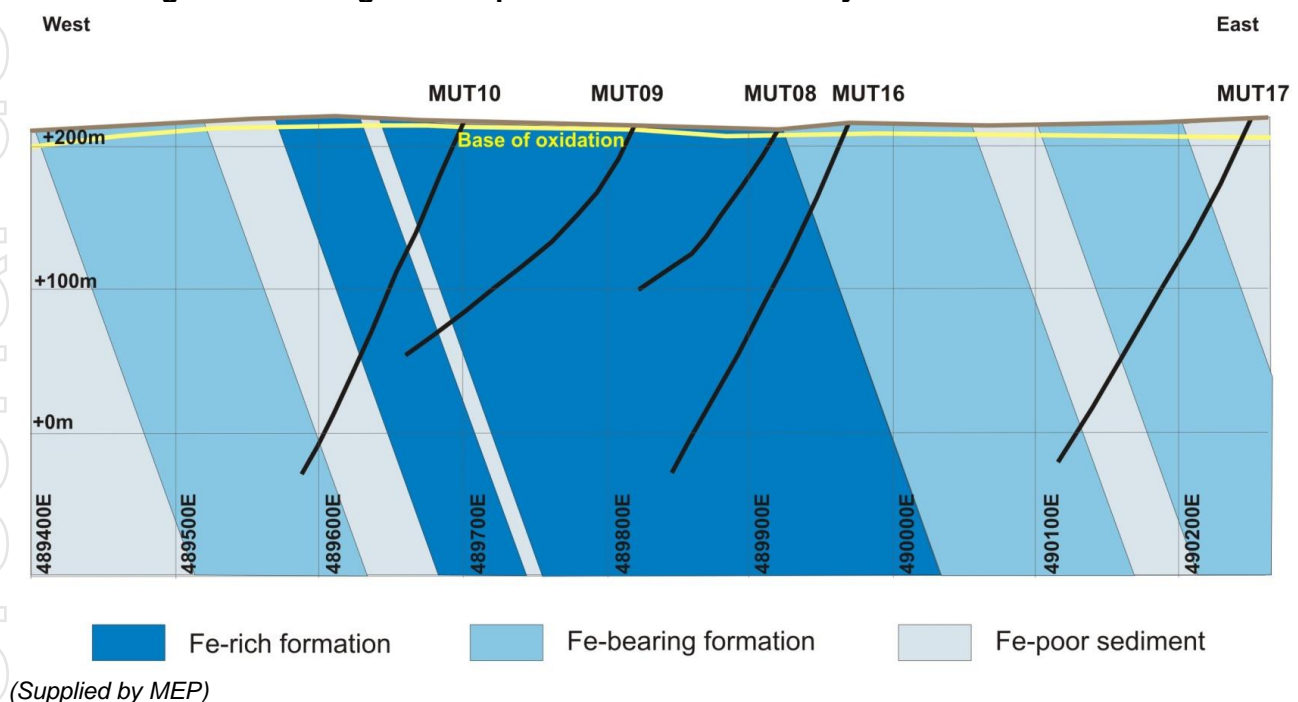
Figure 3 Geological Interpretation of the Discovery Section at Muster Dam
